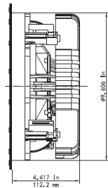
MOUNTING DEPTH/ MINIMUM CUTOUT
