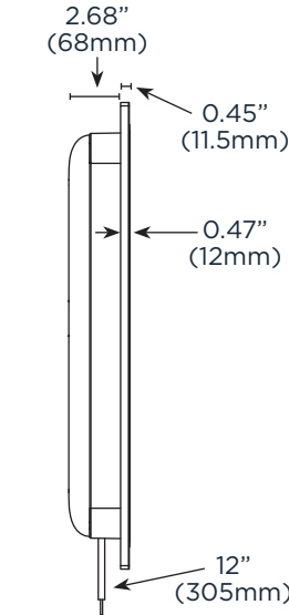
IS8 Side View
