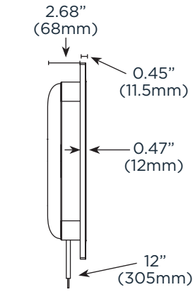
IS6 Side View
