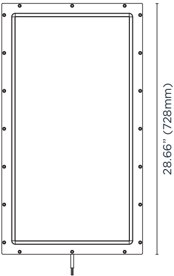
IS10 Front View
